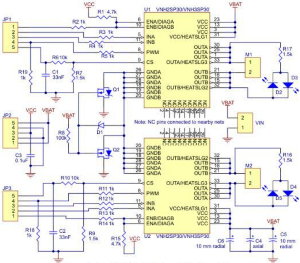
Schematic of the Pololu Dual High Current Motor Driver Carrier
