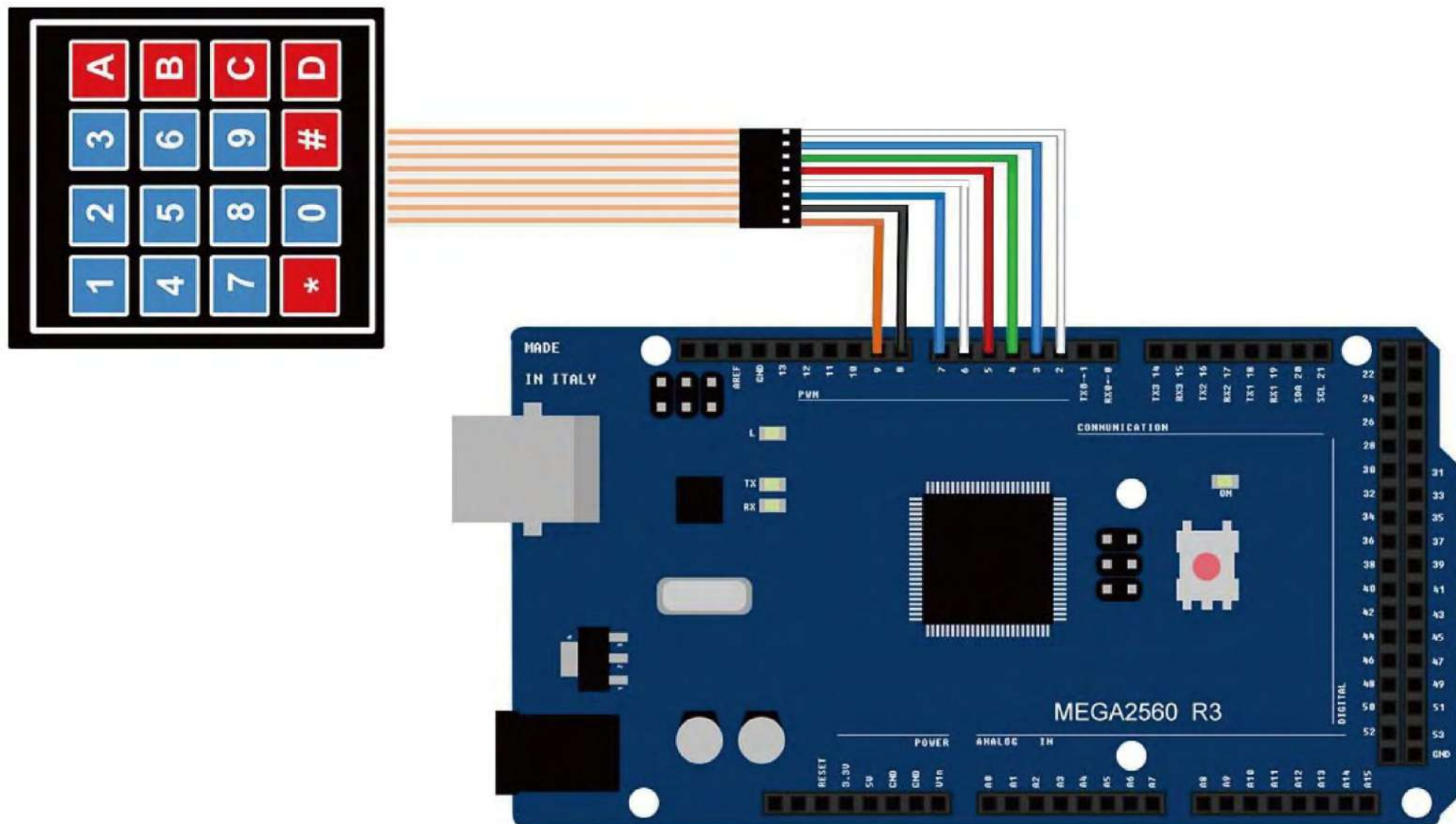
Wiring diagram
