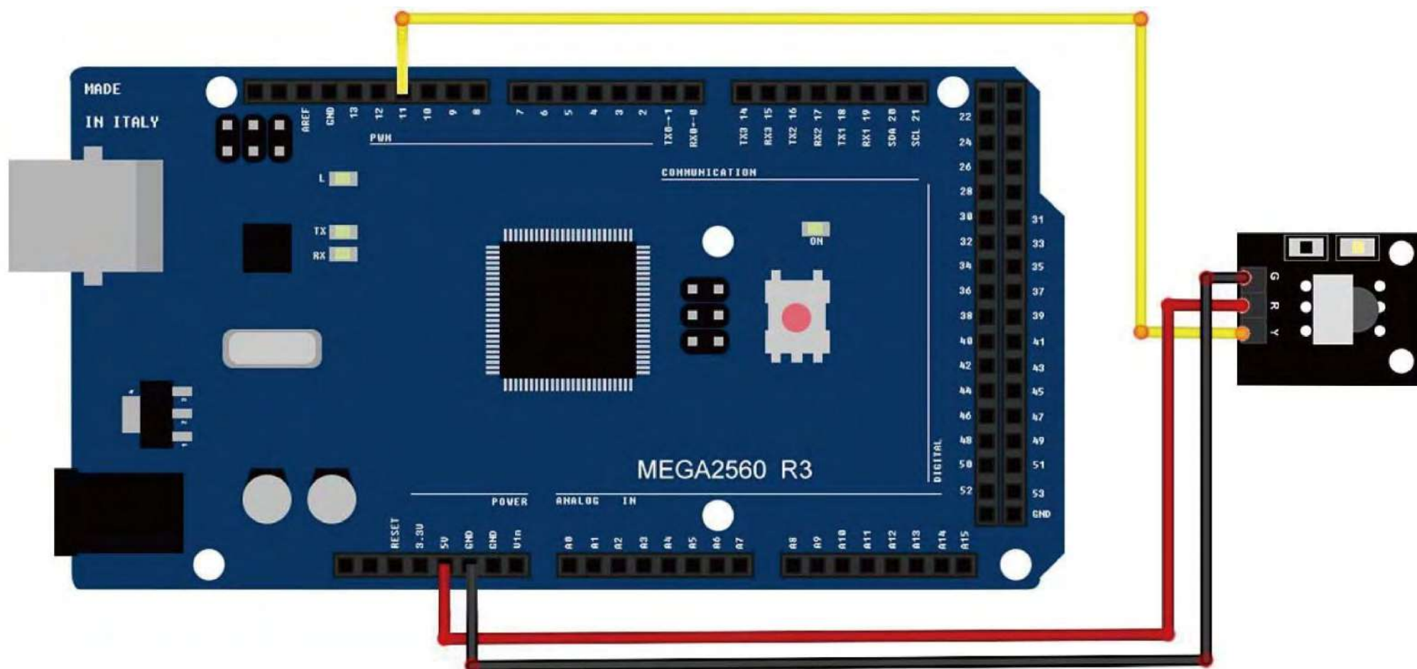
Wiring diagram
