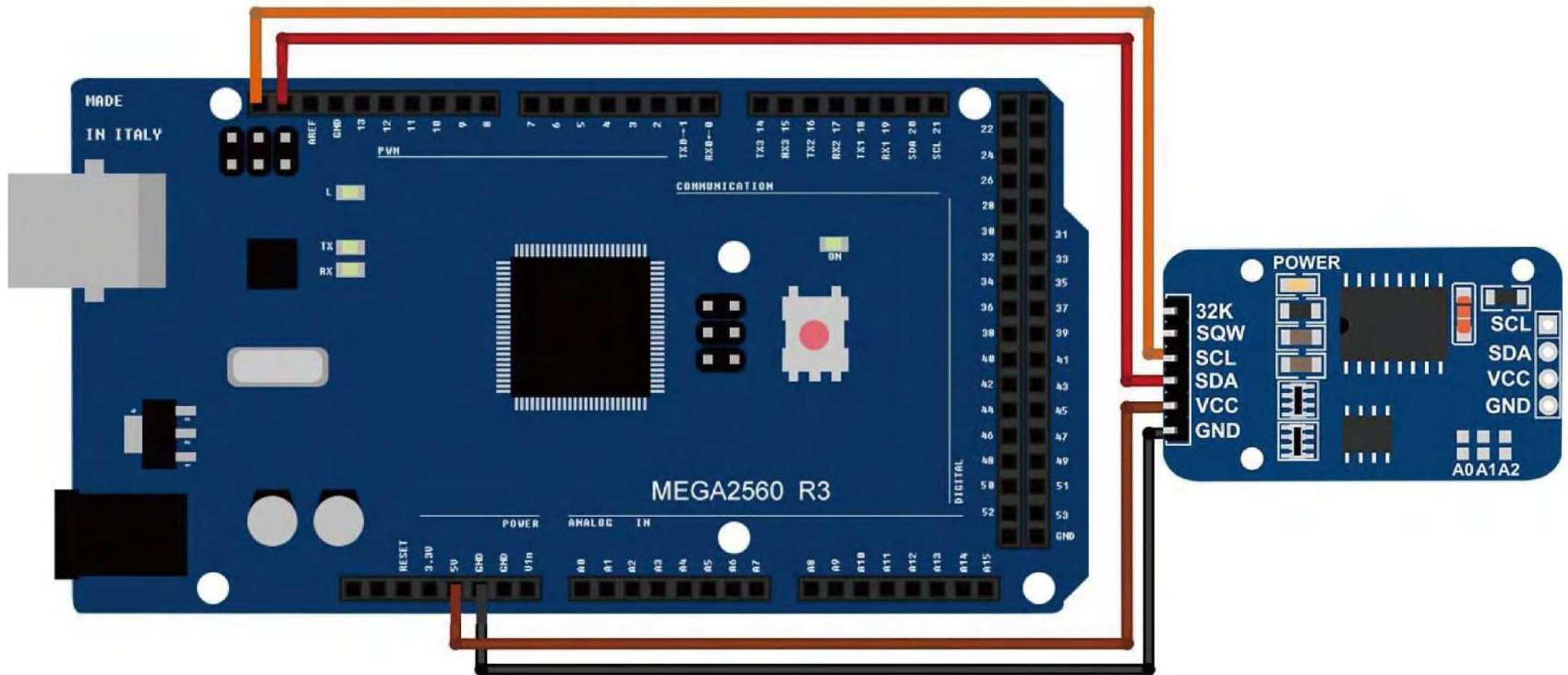
Wiring diagram
