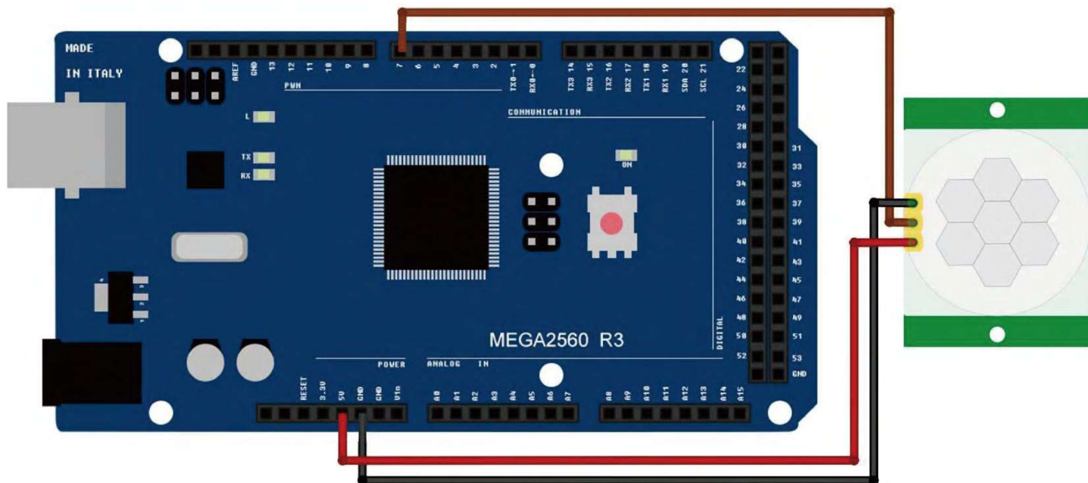
Wiring diagram
