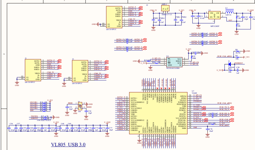
POWER FOR USB 3.0
