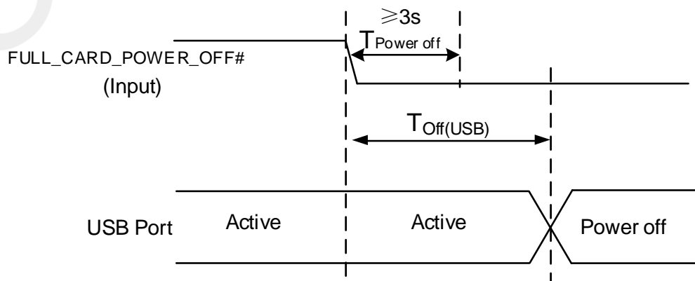
Figure 10: Power off sequence
