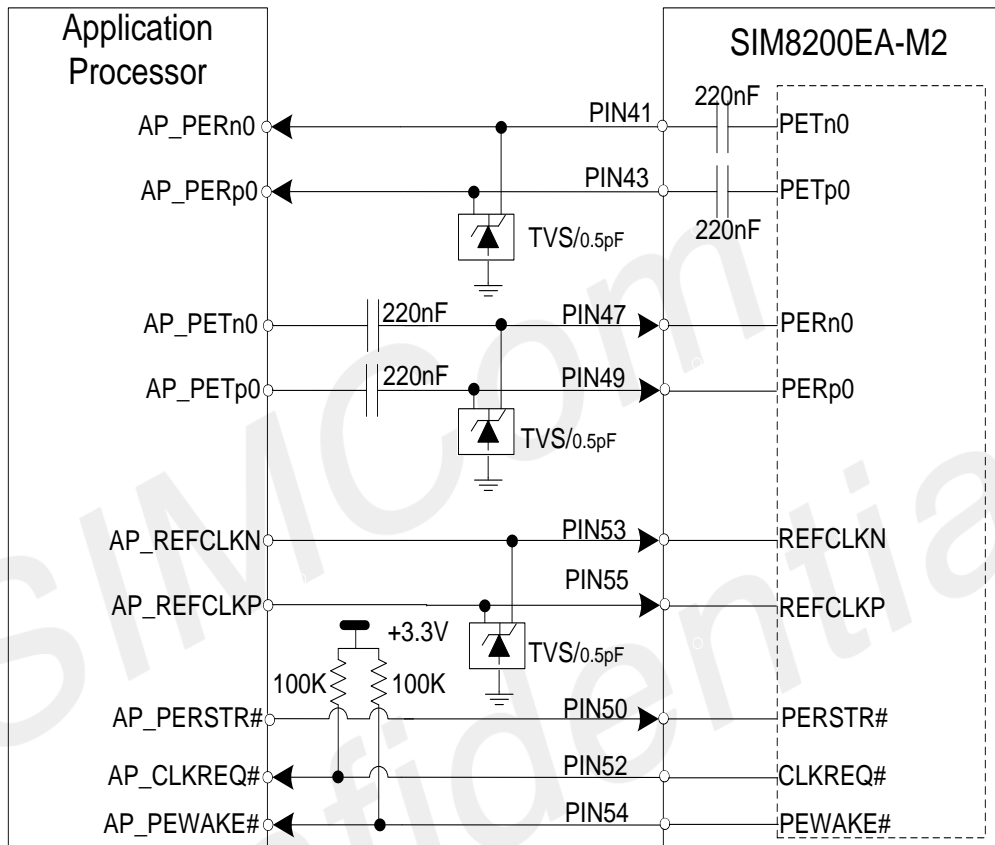
Figure 17: PCIe interface reference circuit (EP Mode)
