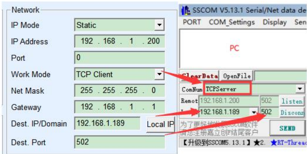
Serial server as a client
