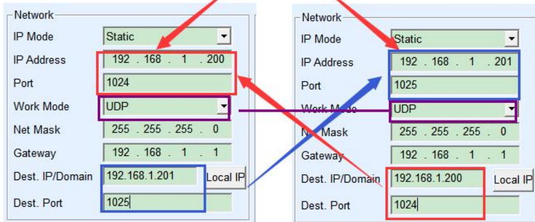
Figure 21 UDP device pairing parameter configuration
